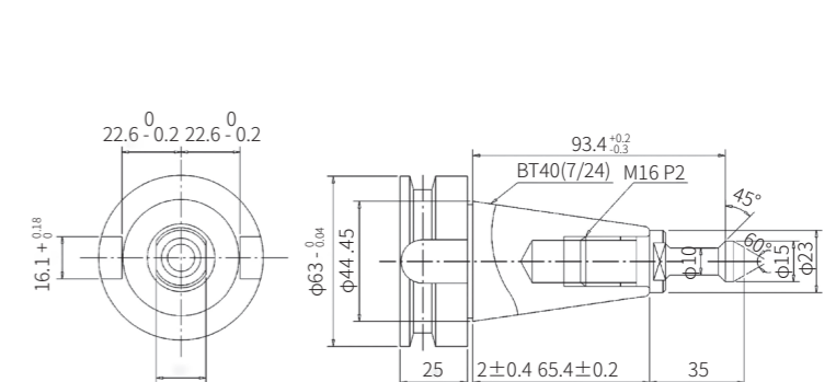
BT40(7: 24) Pull Stud Specification
