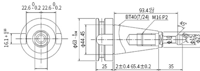
BT40(7: 24) Pull Stud Specification
