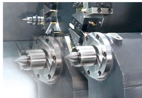
Servo tailstock (For HTC200)
