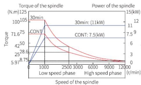
Mitsubishi Electrical Spindle(12000rpm)
